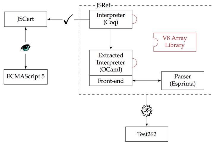
Figure 1: Current Architecture of JSCert
